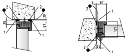
BLOCKZARGE (Standard)
