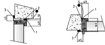
ECKZARGE (Optional)
