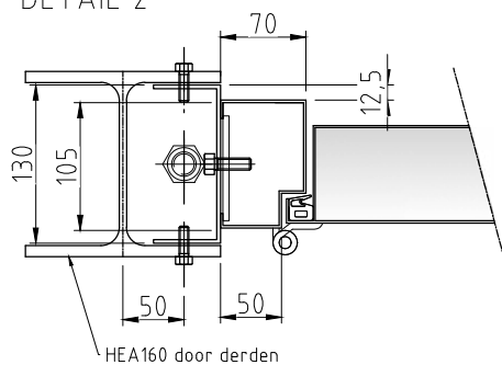
DETAIL 2
